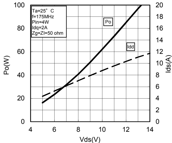
Vds-Po CHARACTERISTICS @f=175MHz
