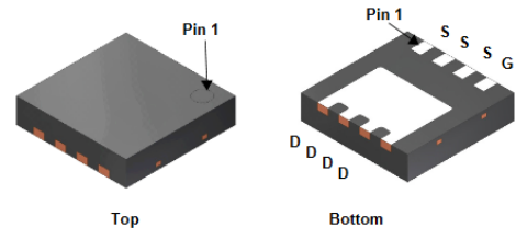
N-CHANNEL MOSFET
