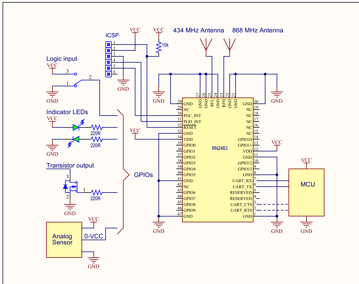
FIGURE 3-1: HARDWARE CONNECTIONS
