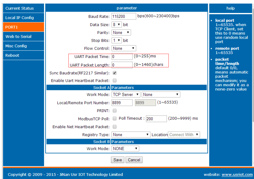
Figure 17 Serial Package
