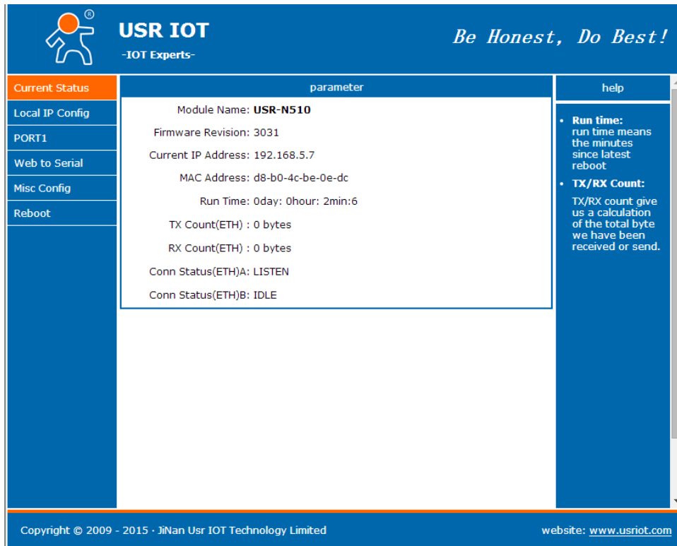
Figure 28 Web Server
