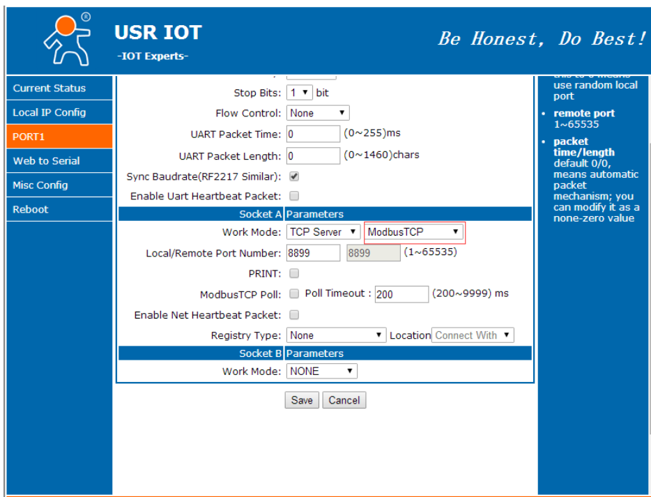
Figure 23 Modbus RTU<=>Modbus TCP
