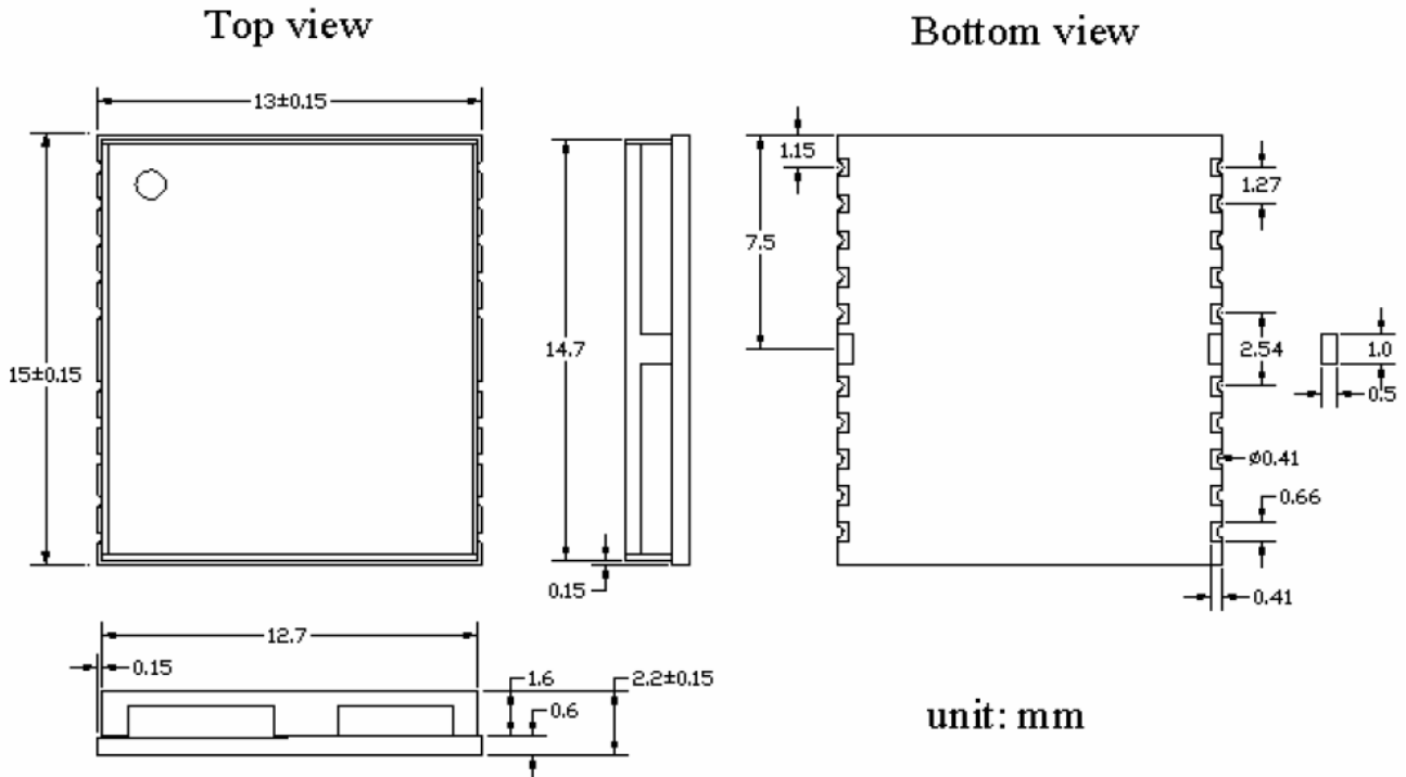
Figure 3: GT-1513-SF Dimensions
