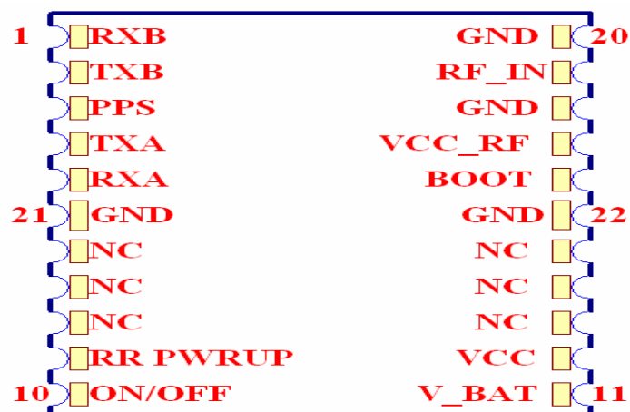
Figure 2: GT-1513-SF Pin Package
