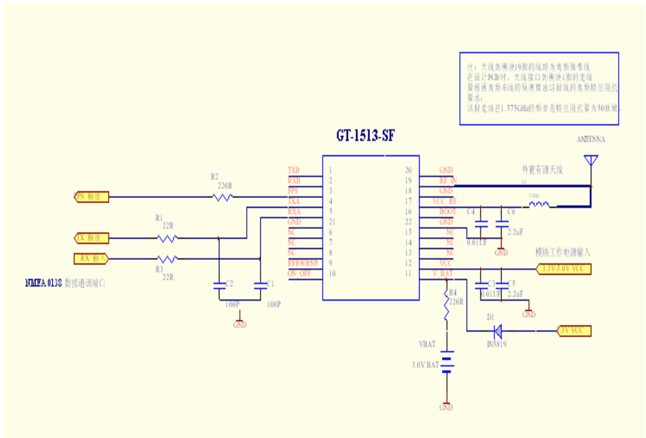
Typical application circuit that uses active antenna
